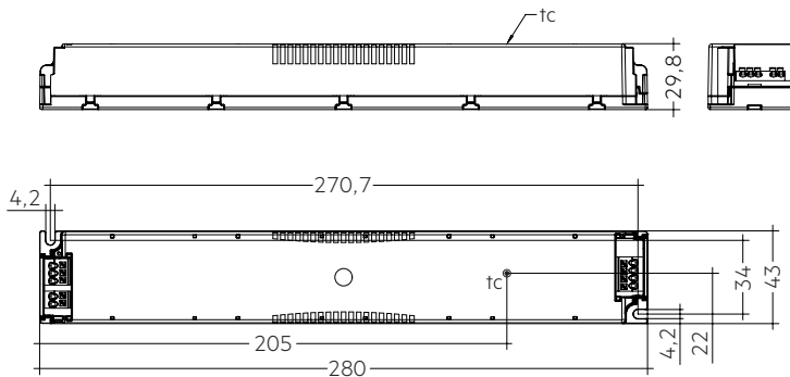
Without strain-relief
